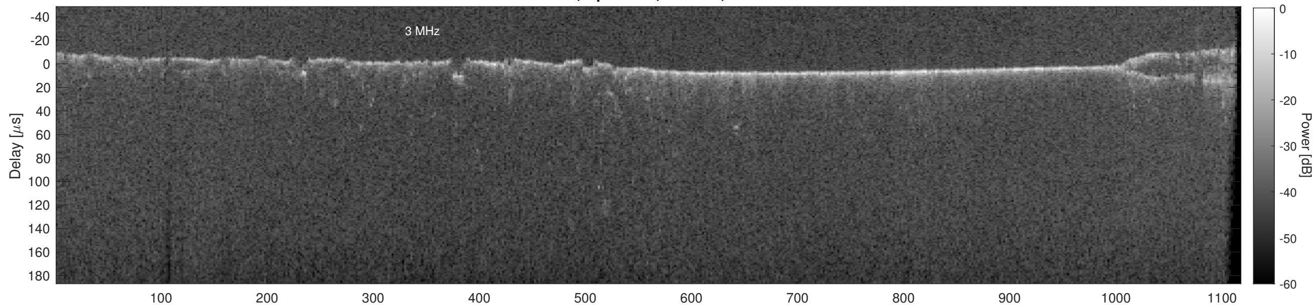
Orbit 18458, Cluttergram
