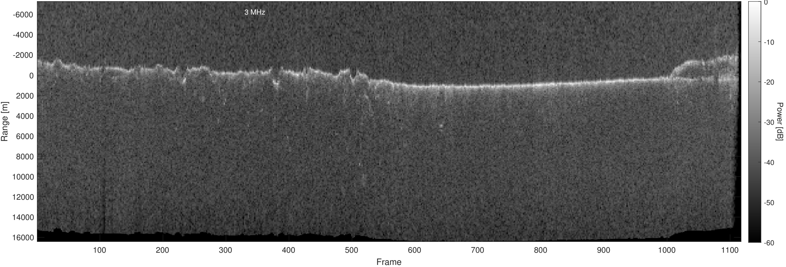
Orbit 18458, Optimized, Window, Depth-Corrected, Channel 2
