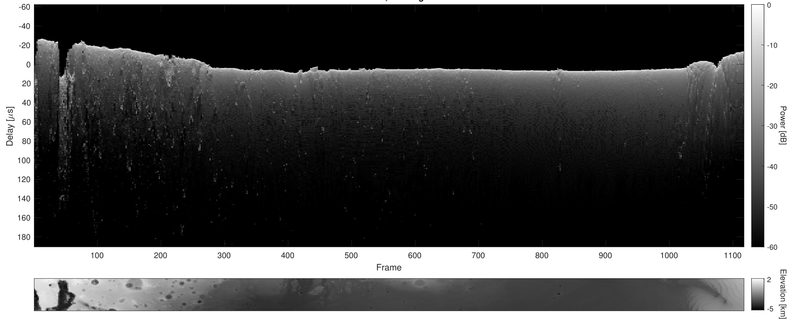
Orbit 18462, Cluttergram
