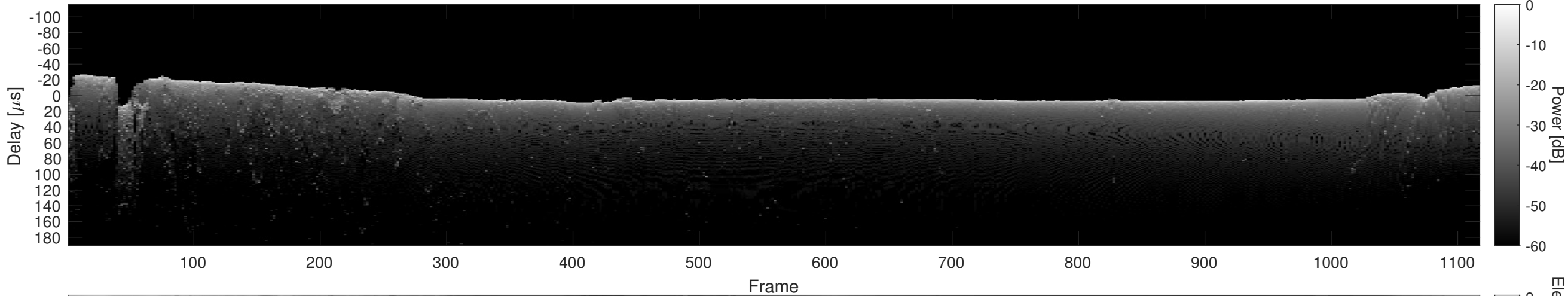
Orbit 18462, Cluttergram
