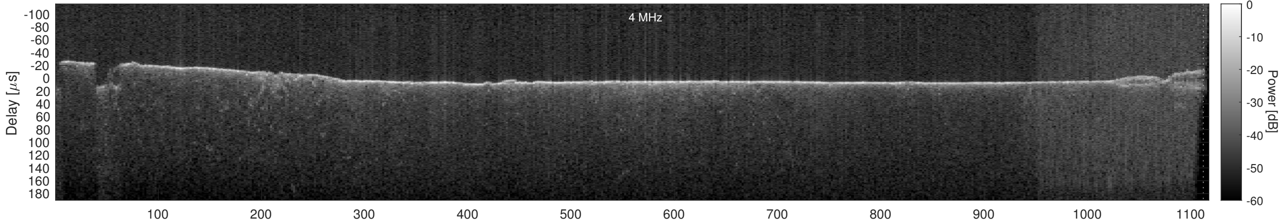
Orbit 18462, Cluttergram
