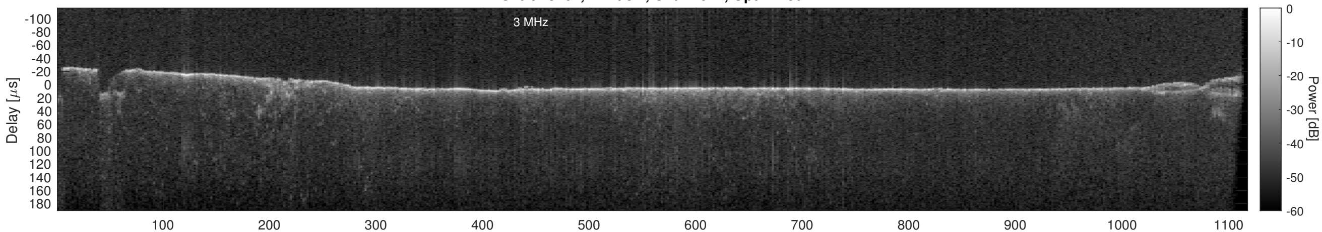
Orbit 18462, Cluttergram
