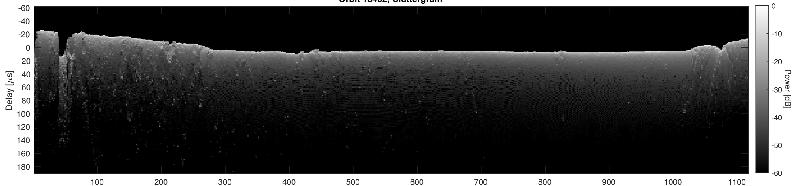
Orbit 18462, Cluttergram
