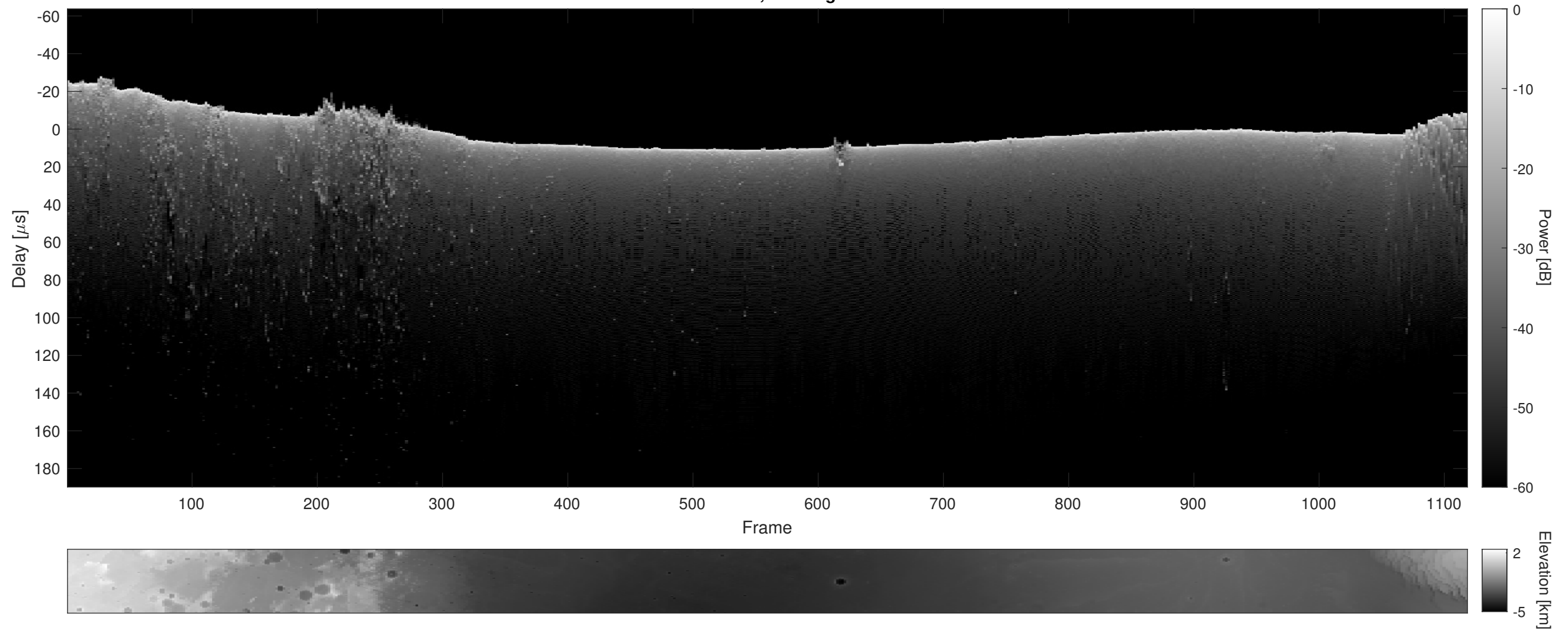
Orbit 18464, Cluttergram
