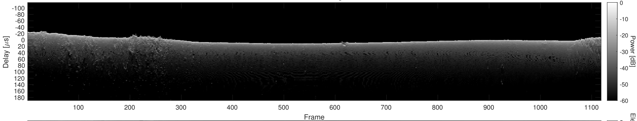
Orbit 18464, Cluttergram
