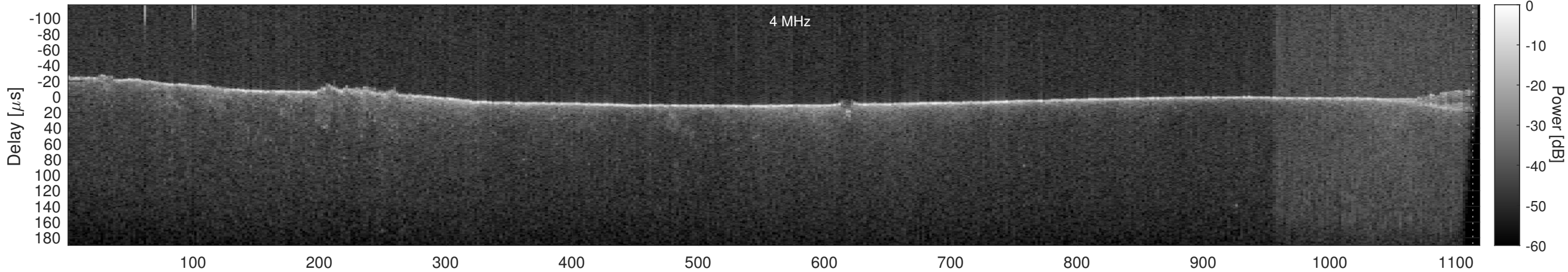
Orbit 18464, Cluttergram
