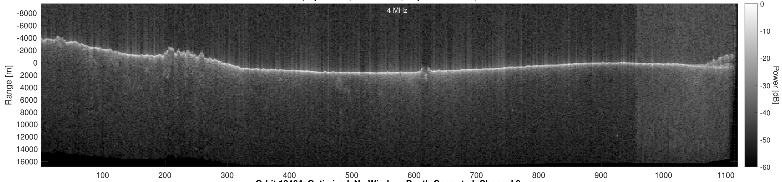
Orbit 18464, Optimized, No Window, Depth-Corrected, Channel 2
