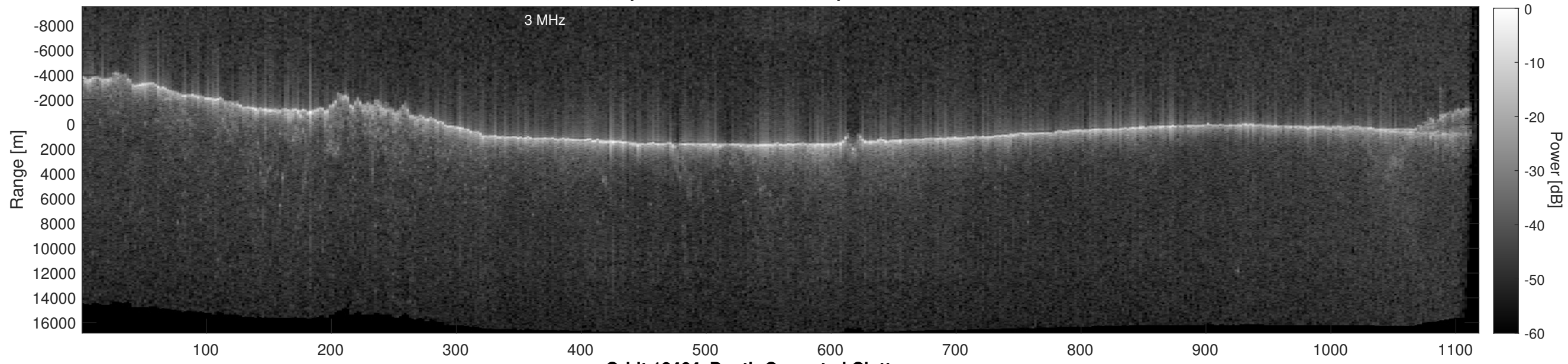
Orbit 18464, Depth-Corrected Cluttergram
