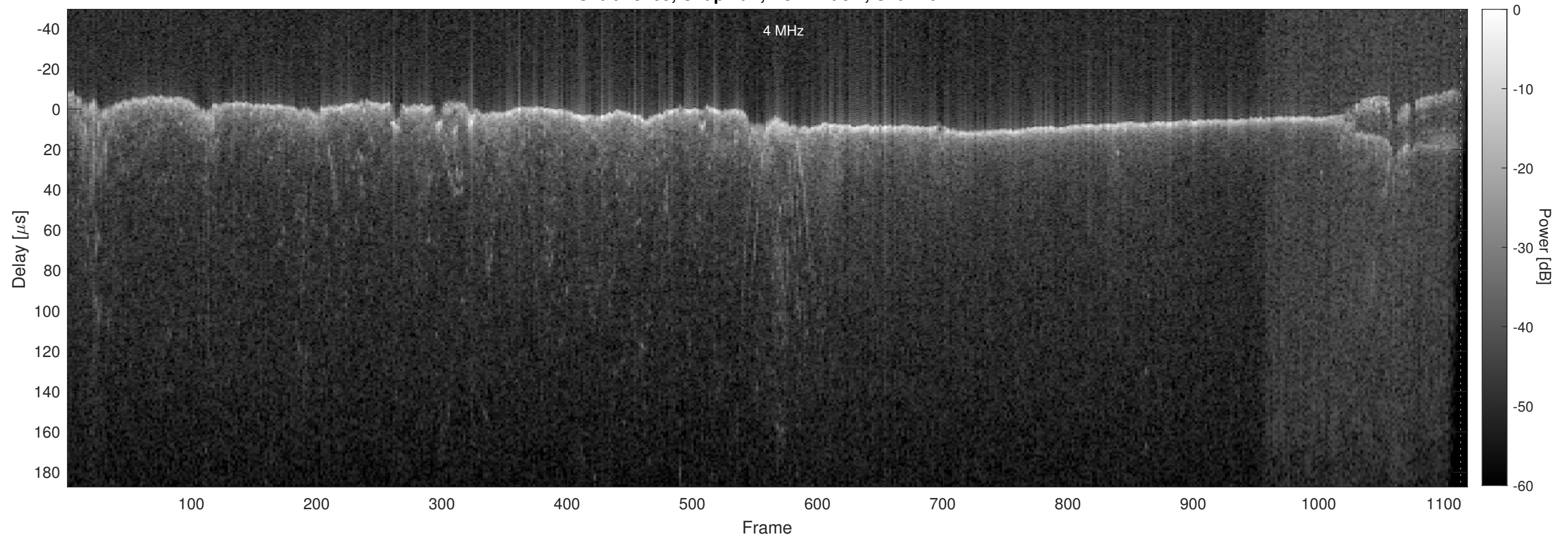
Orbit 18465, Chapman, No Window, Channel 2
