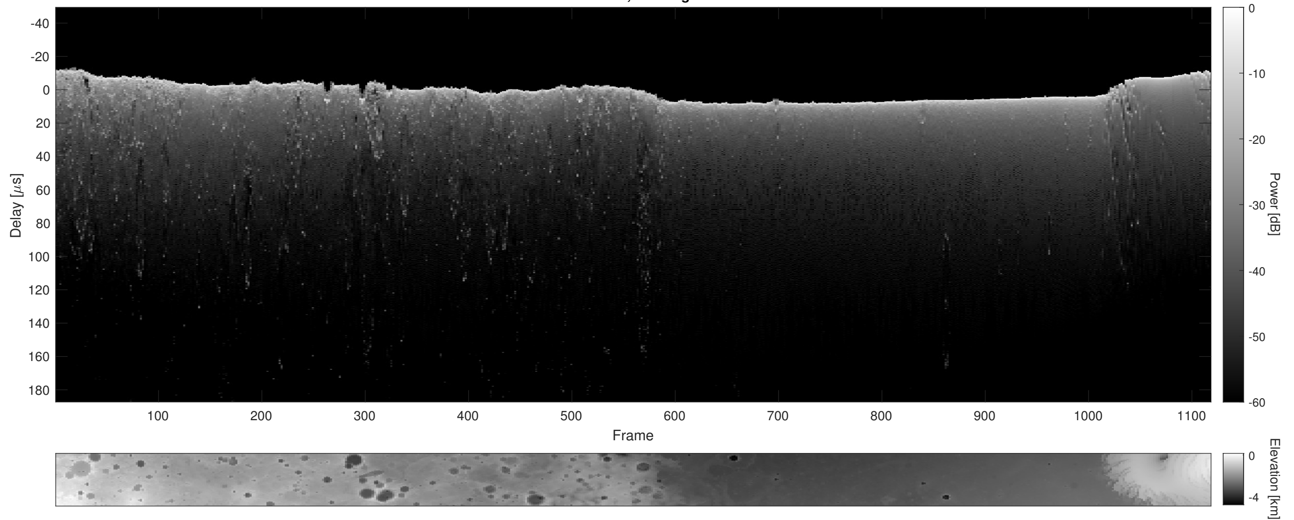
Orbit 18465, Cluttergram
