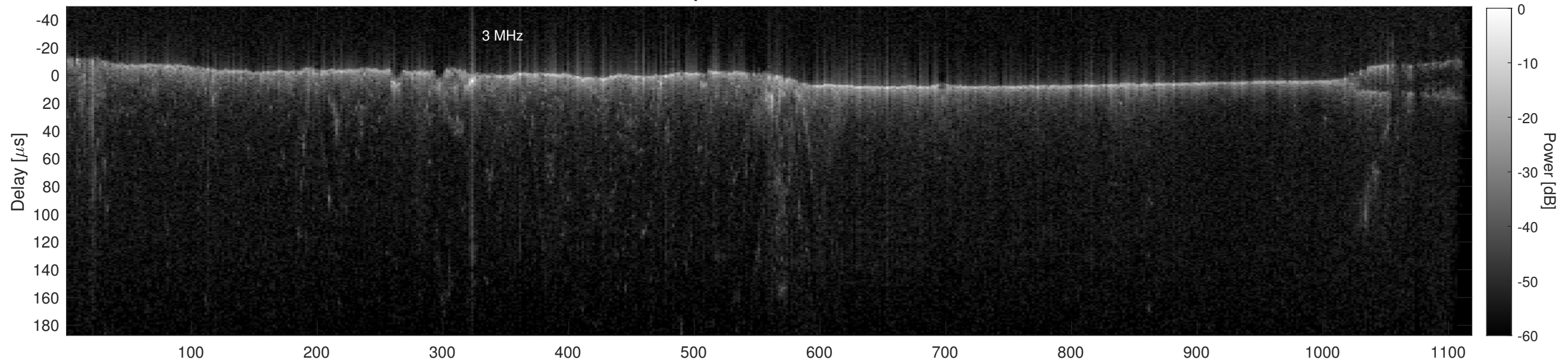
Orbit 18465, Cluttergram
