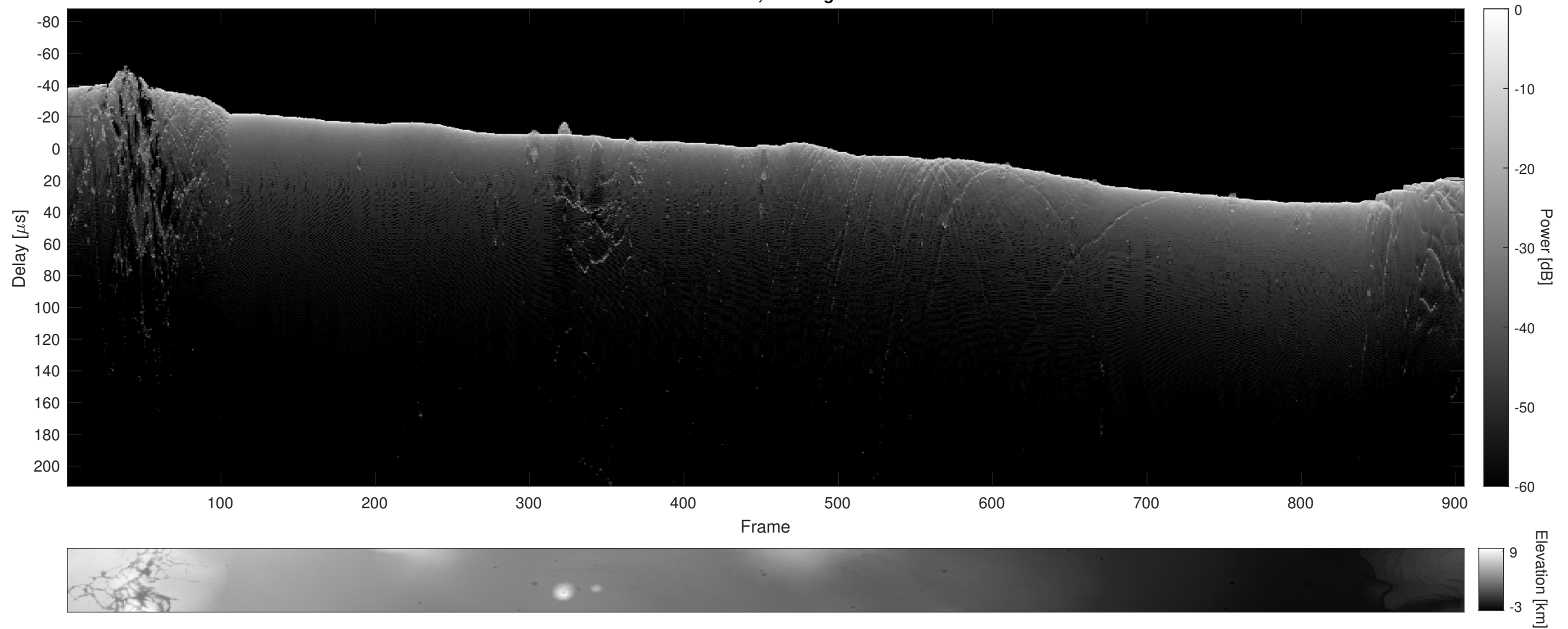
Orbit 18466, Cluttergram
