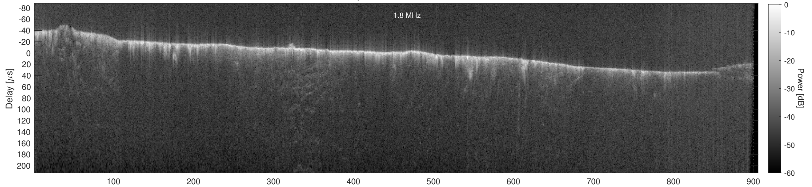
Orbit 18466, Cluttergram
