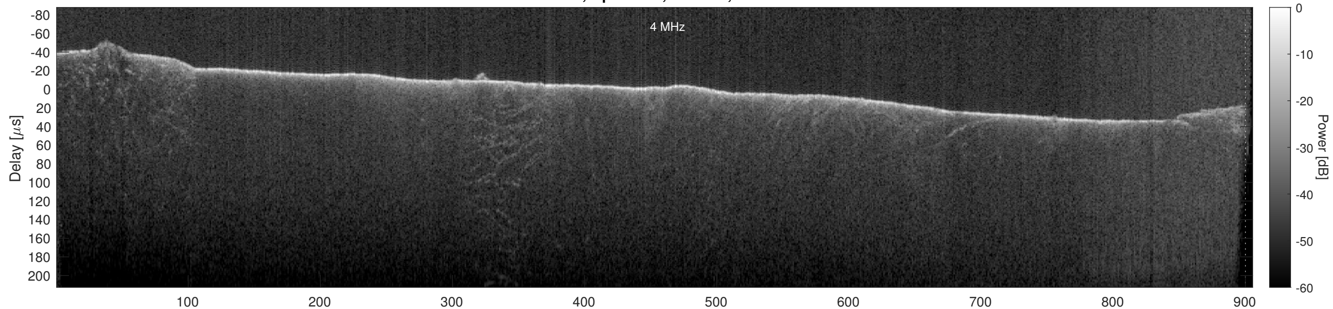
Orbit 18466, Optimized, Window, Channel 2
