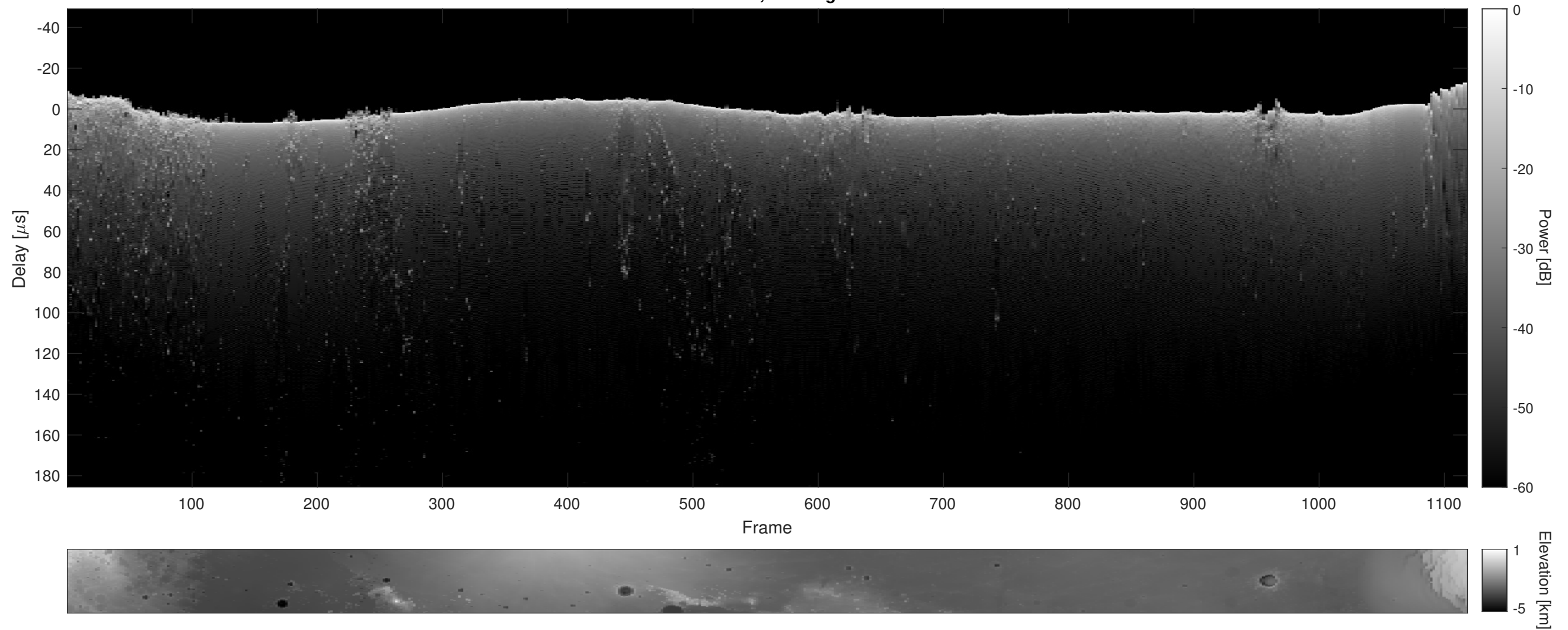
Orbit 18467, Cluttergram
