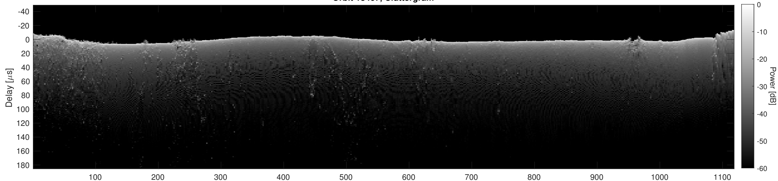
Orbit 18467, Cluttergram
