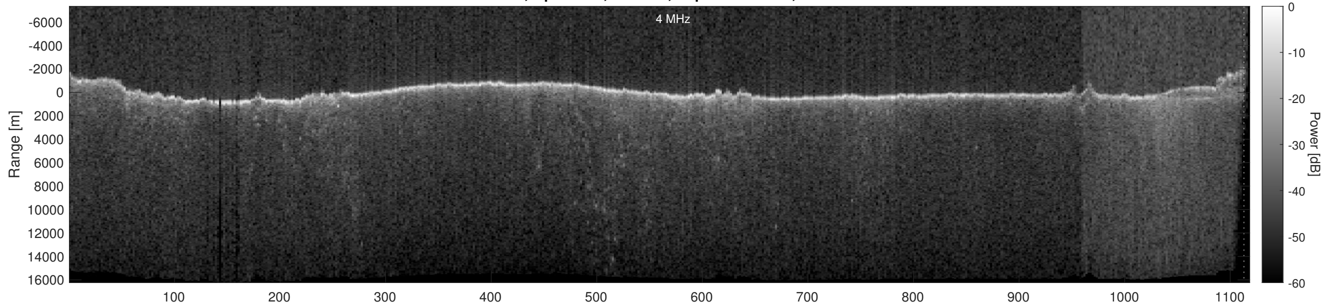
Orbit 18467, Optimized, Window, Depth-Corrected, Channel 2
