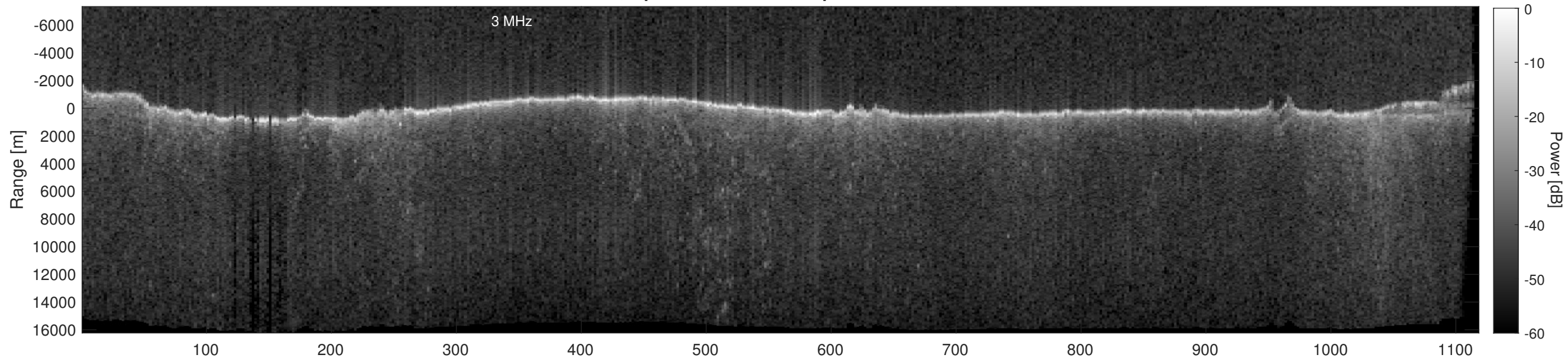
Orbit 18467, Depth-Corrected Cluttergram
