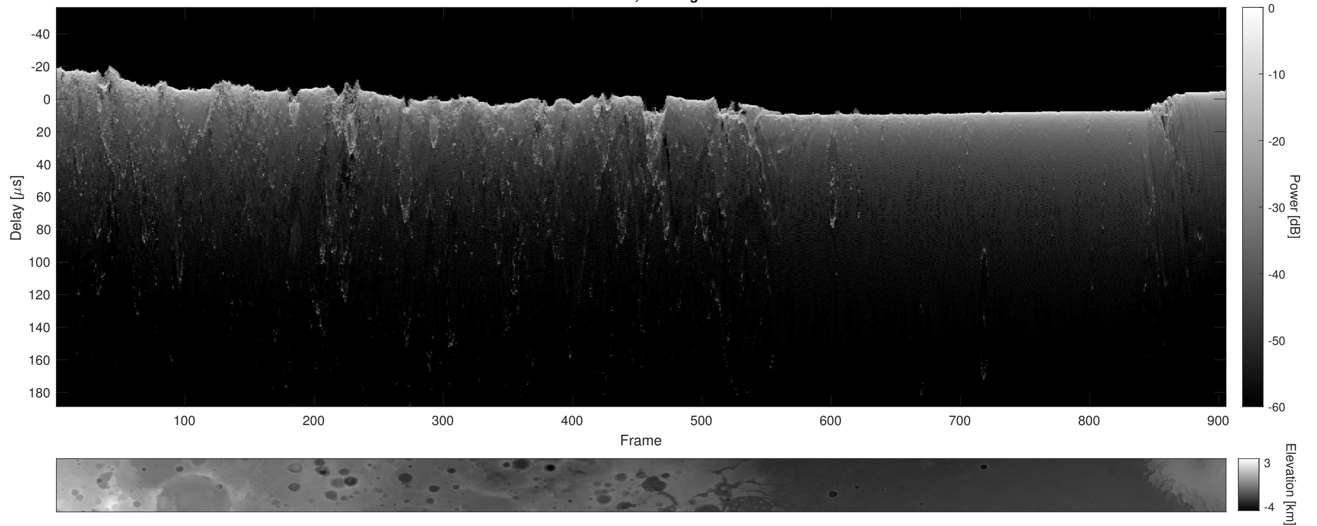
Orbit 18479, Cluttergram
