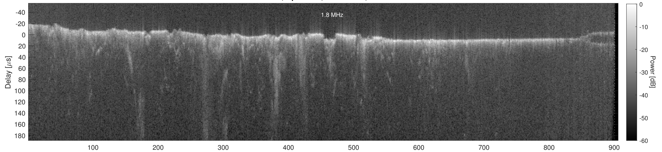
Orbit 18479, Cluttergram
