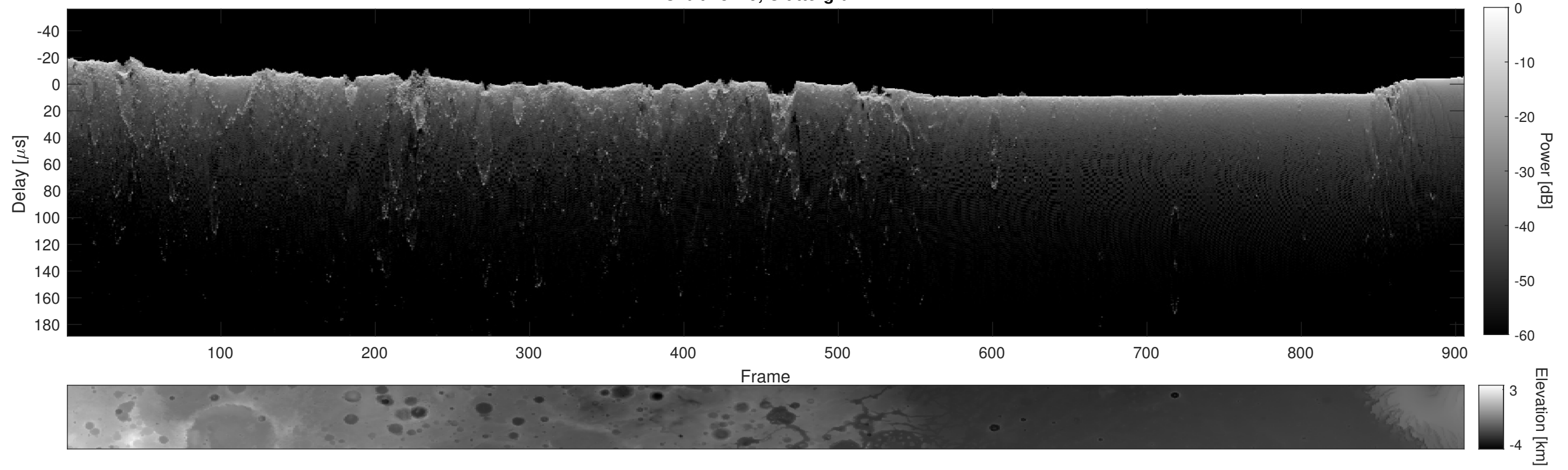
Orbit 18479, Cluttergram
