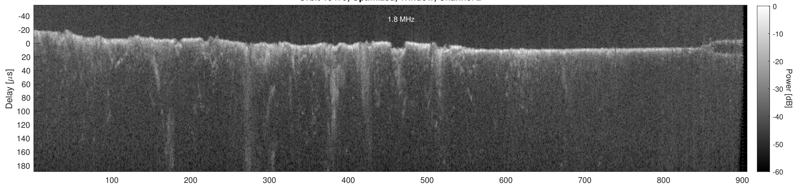
Orbit 18479, Cluttergram
