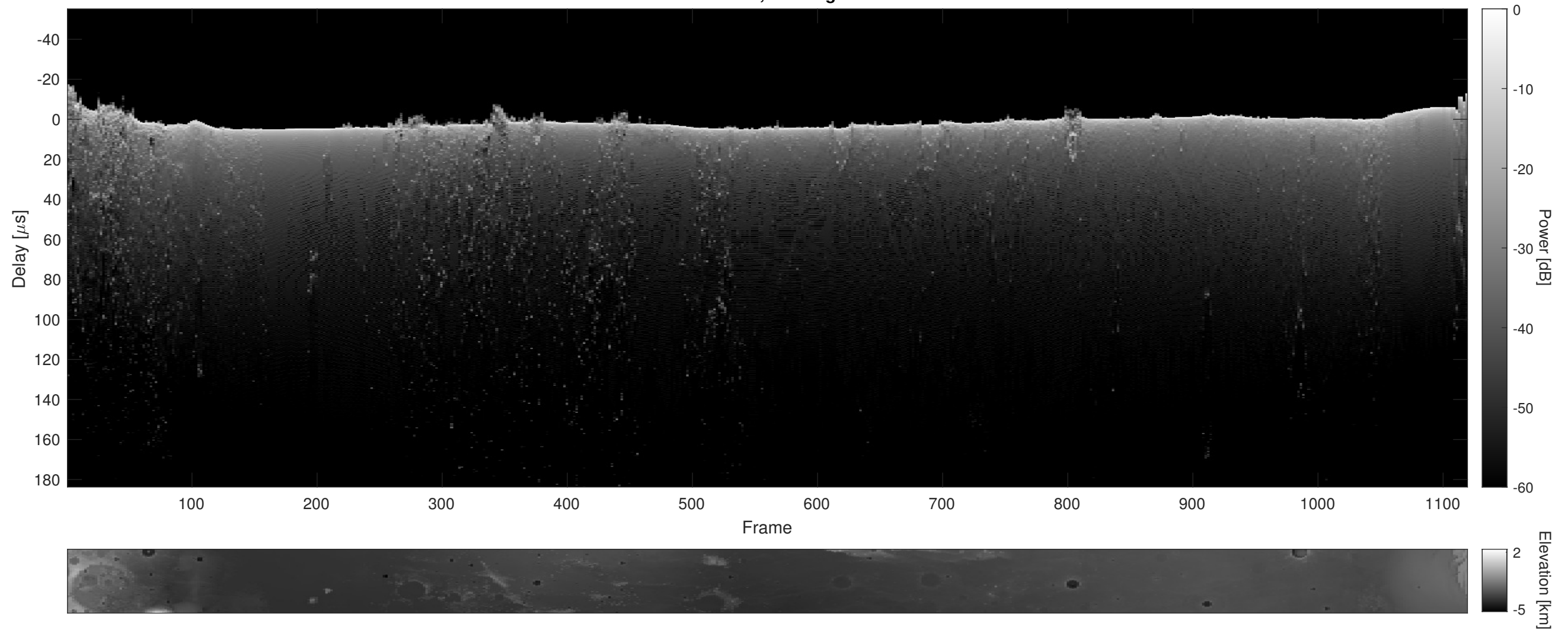
Orbit 18481, Cluttergram
