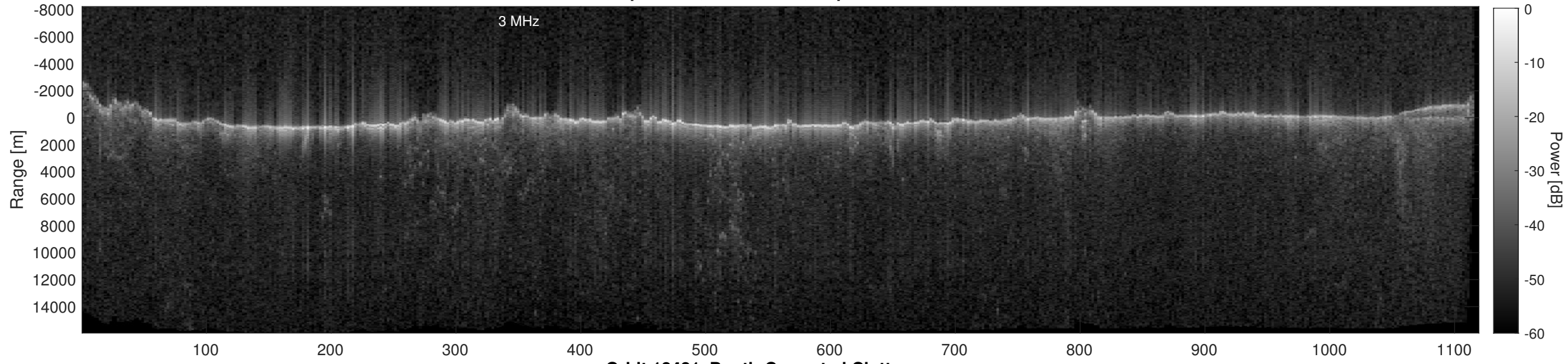
Orbit 18481, Depth-Corrected Cluttergram
