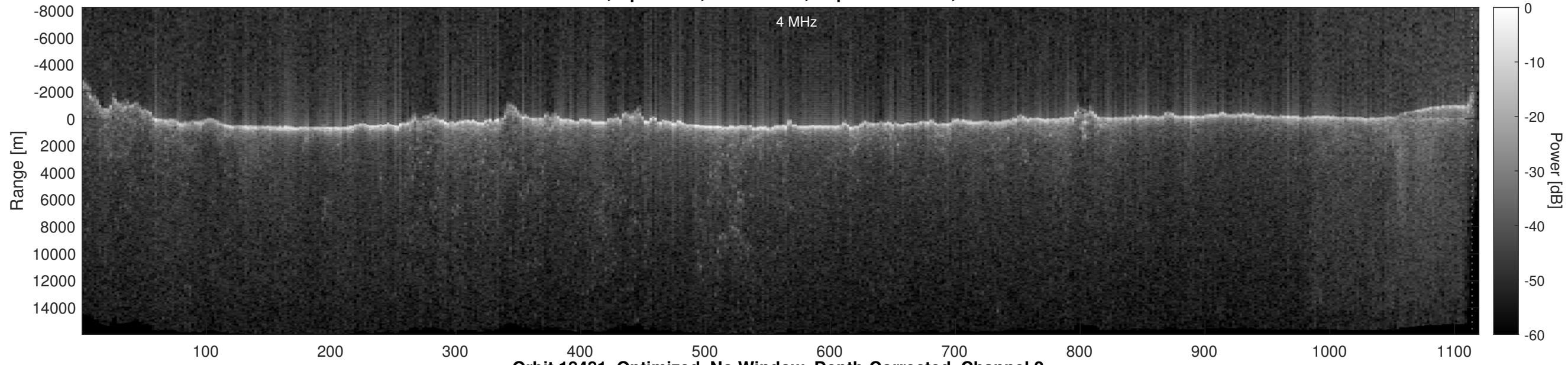
Orbit 18481, Optimized, No Window, Depth-Corrected, Channel 2
