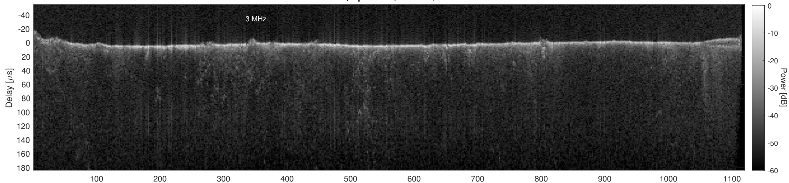
Orbit 18481, Cluttergram
