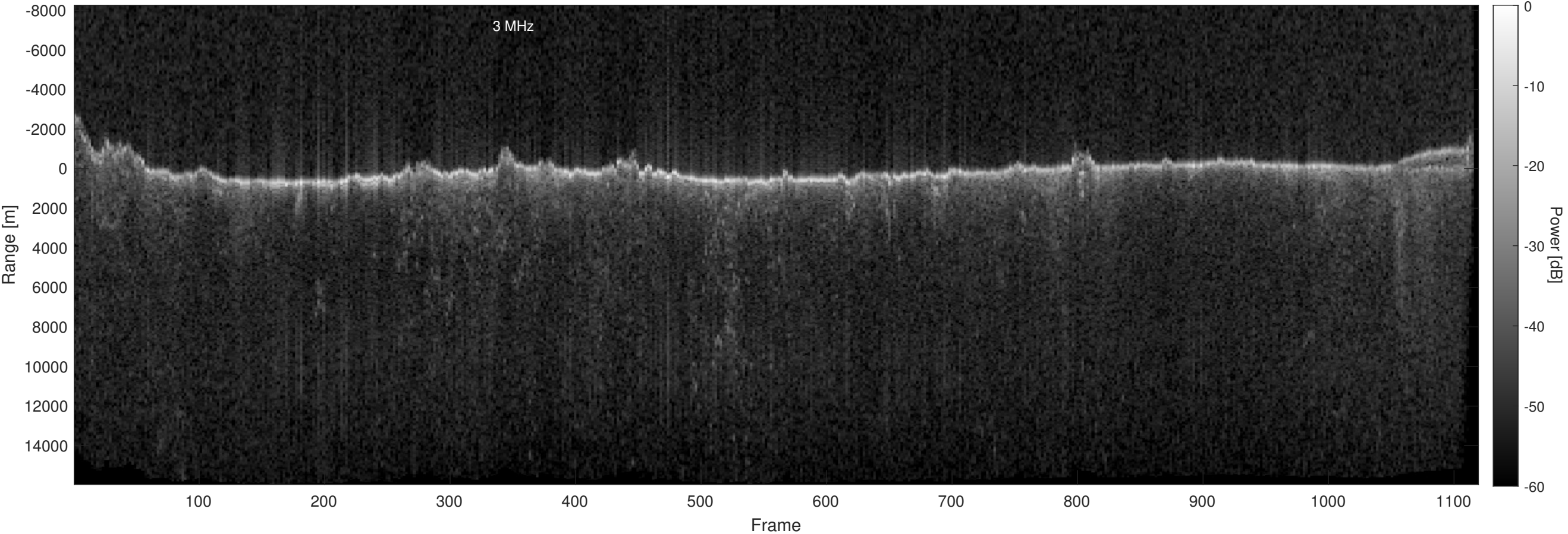
Orbit 18481, Optimized, Window, Depth-Corrected, Channel 2
