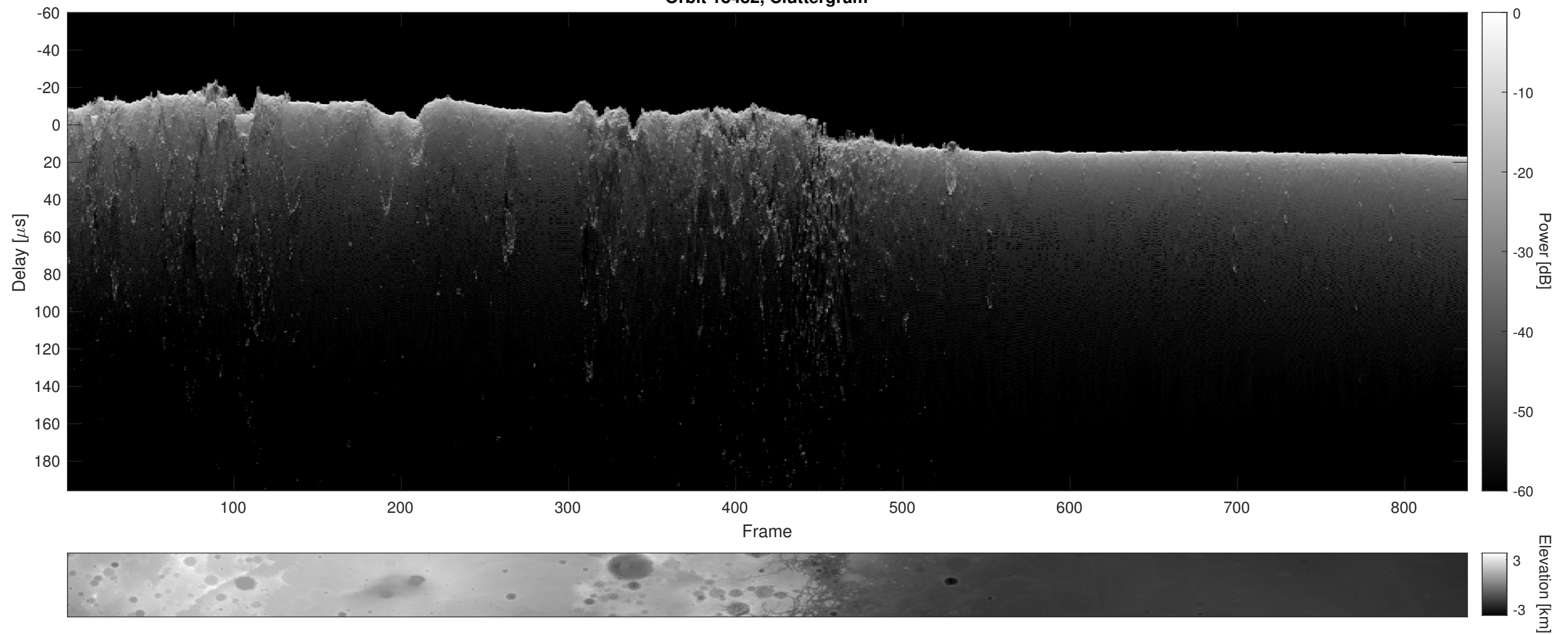
Orbit 18482, Cluttergram
