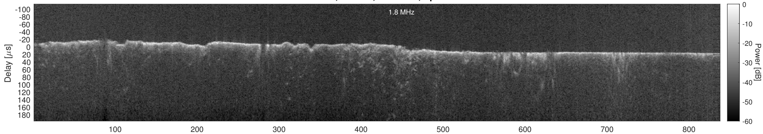
Orbit 18482, Cluttergram
