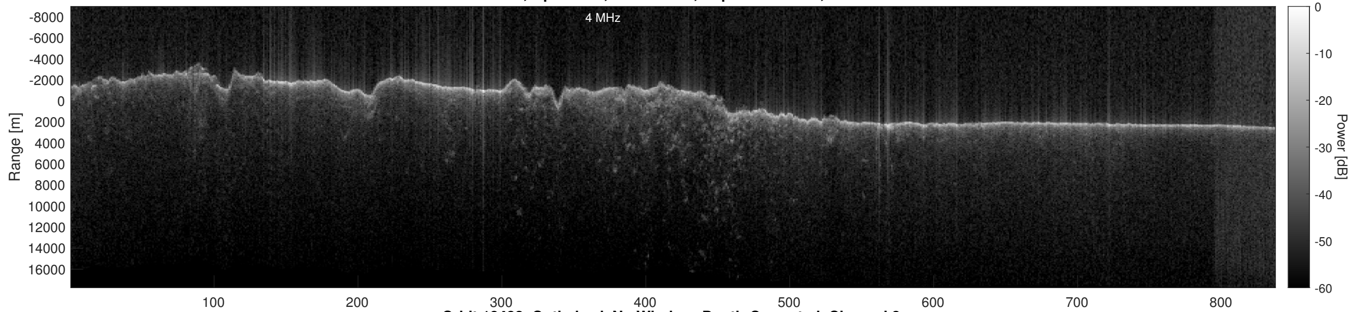
Orbit 18482, Optimized, No Window, Depth-Corrected, Channel 2
