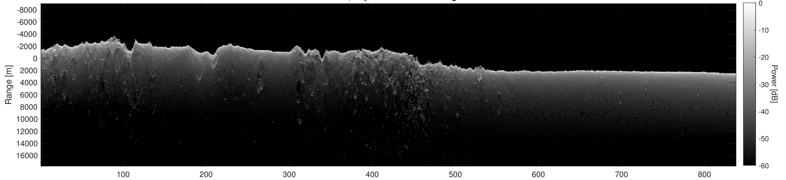
Orbit 18482, Depth-Corrected Cluttergram
