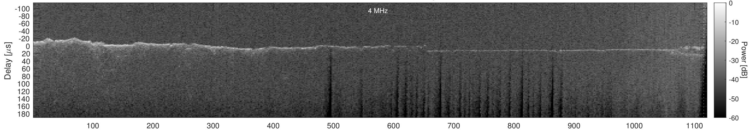
Orbit 18486, Window, Channel 1, Optimized
