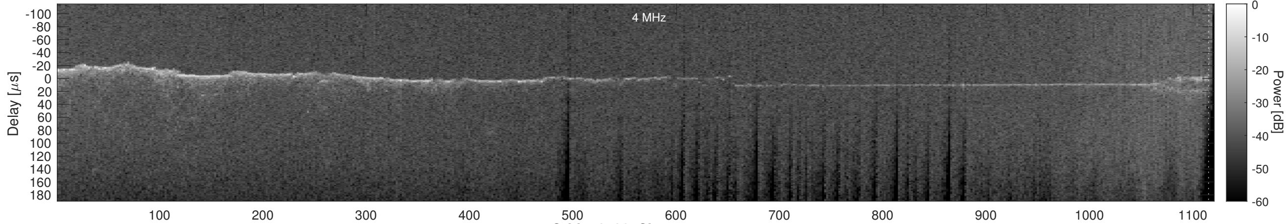
Orbit 18486, Cluttergram
