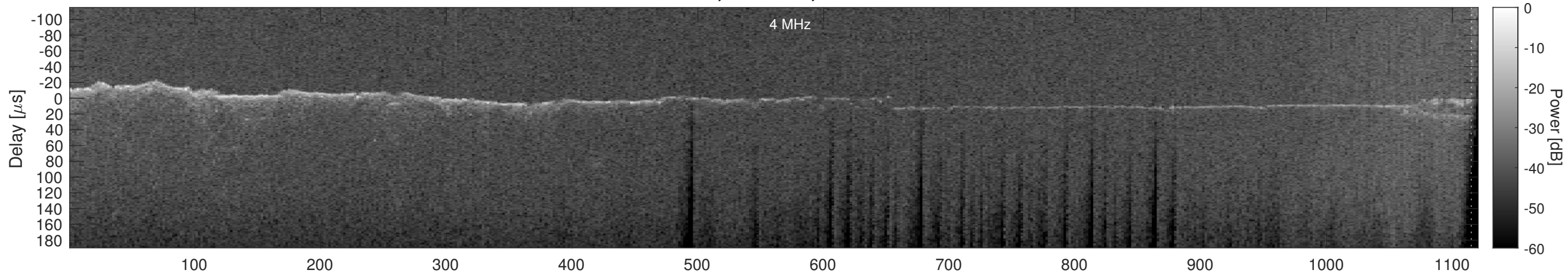
Orbit 18486, Window, Channel 1, Chapman
