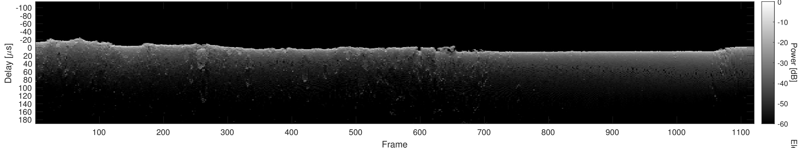
Orbit 18486, Cluttergram
