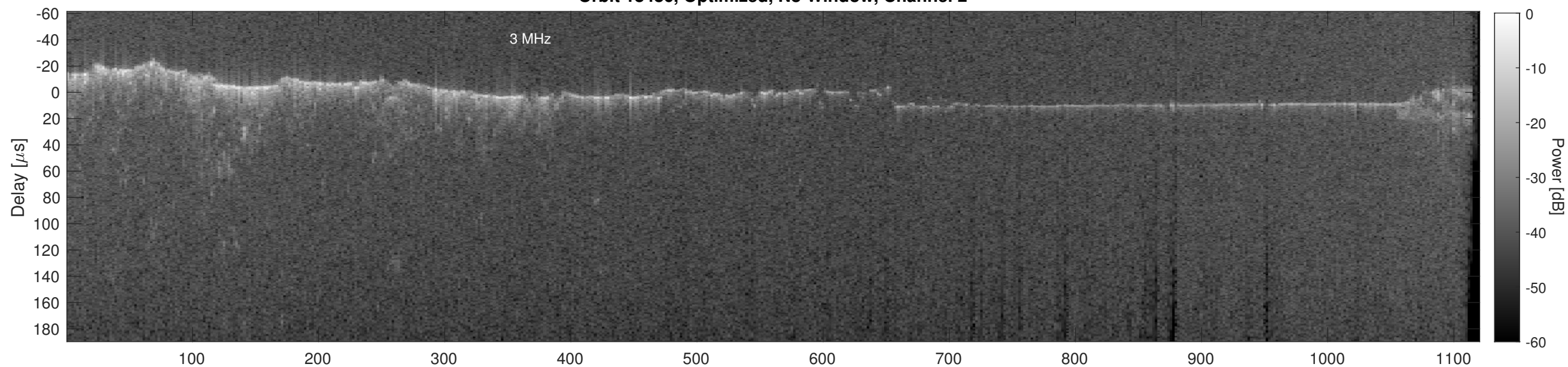
Orbit 18486, Cluttergram
