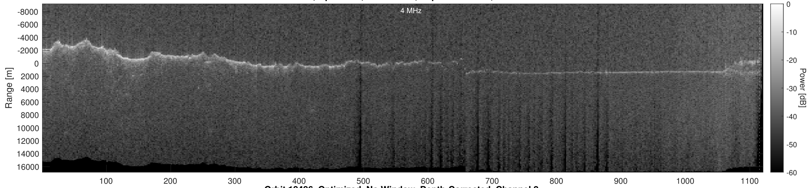
Orbit 18486, Optimized, No Window, Depth-Corrected, Channel 2
