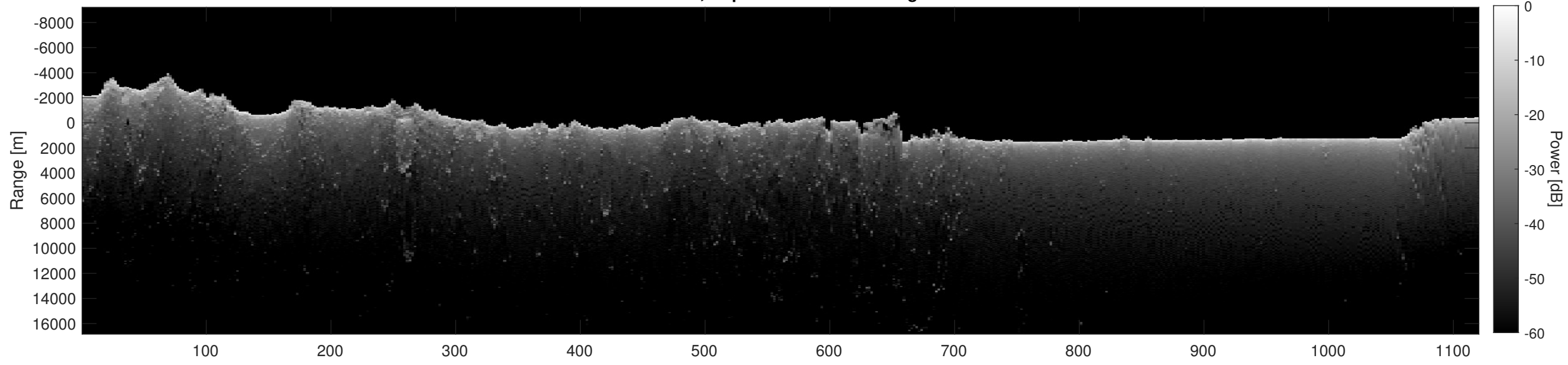
Orbit 18486, Depth-Corrected Cluttergram
