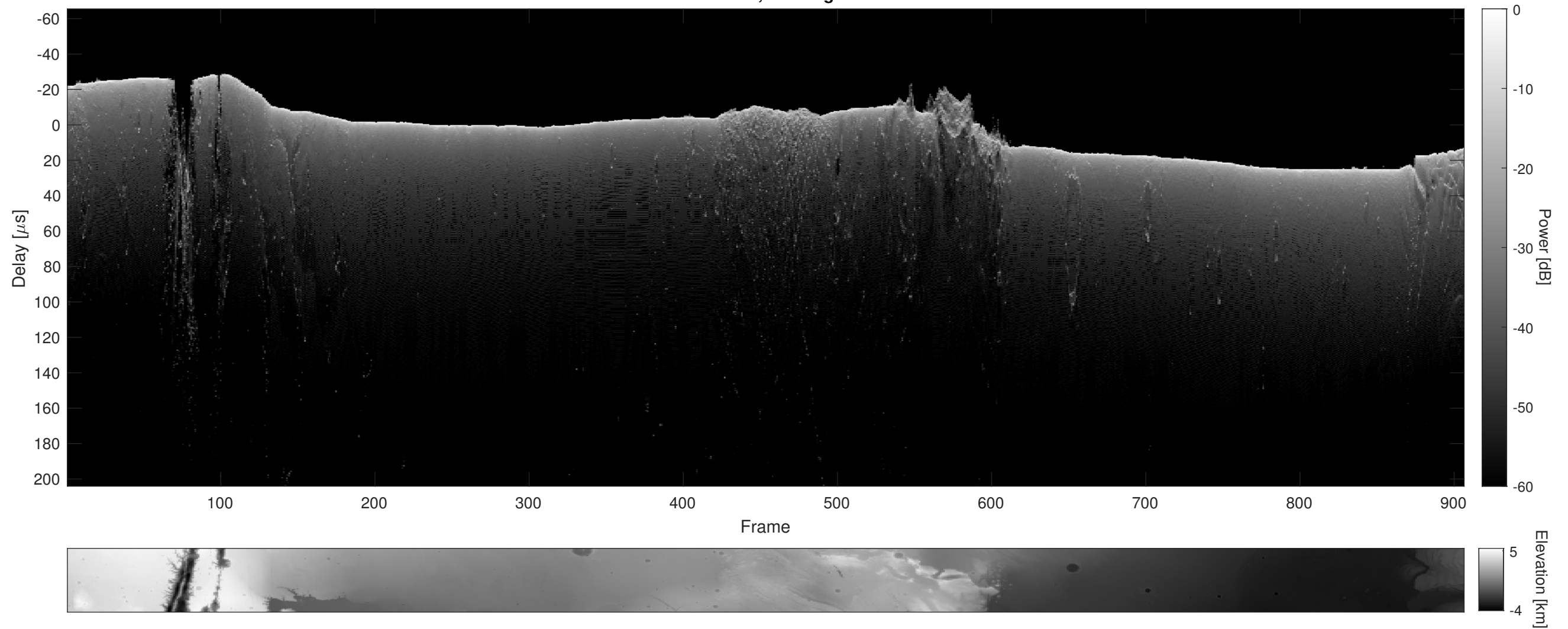
Orbit 18487, Cluttergram
