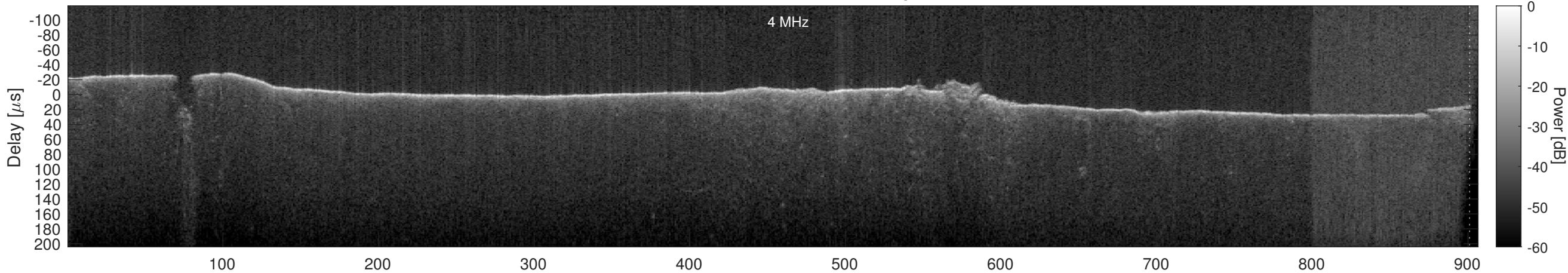
Orbit 18487, Window, Channel 1, Optimized
