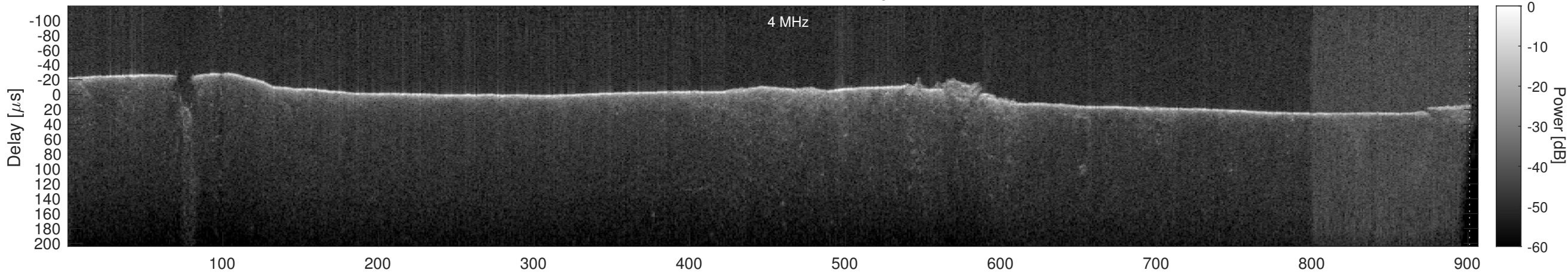
Orbit 18487, Cluttergram
