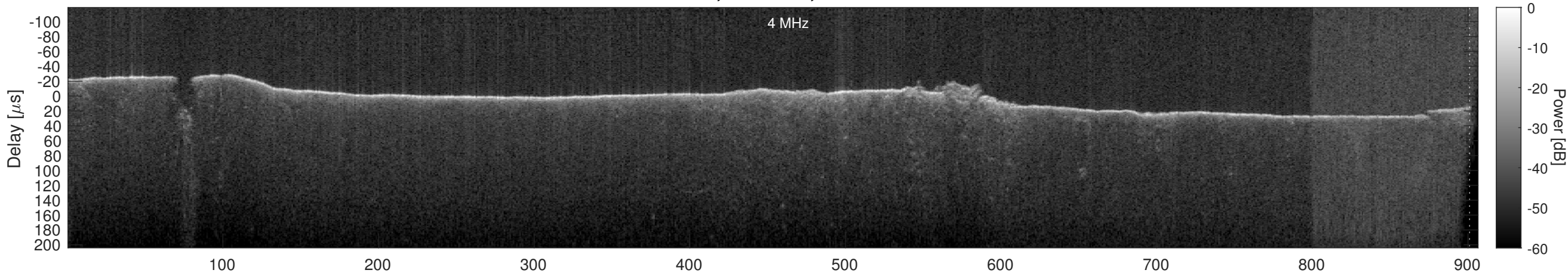
Orbit 18487, Window, Channel 1, Chapman
