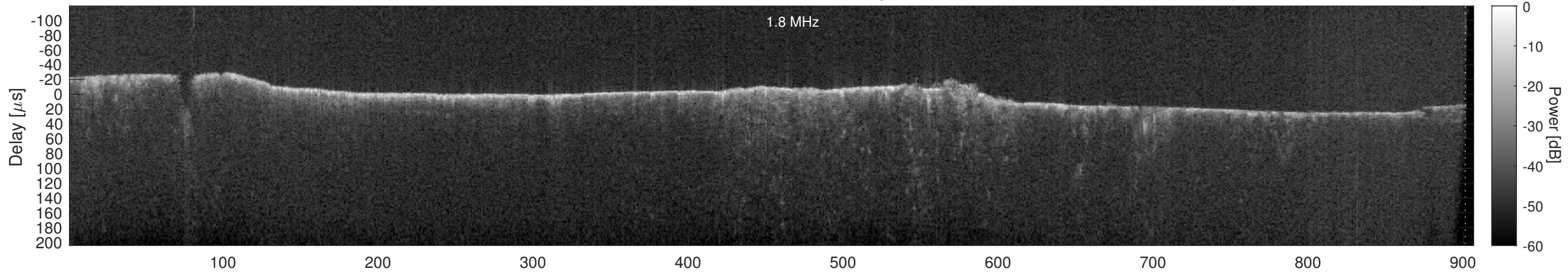
Orbit 18487, Cluttergram
