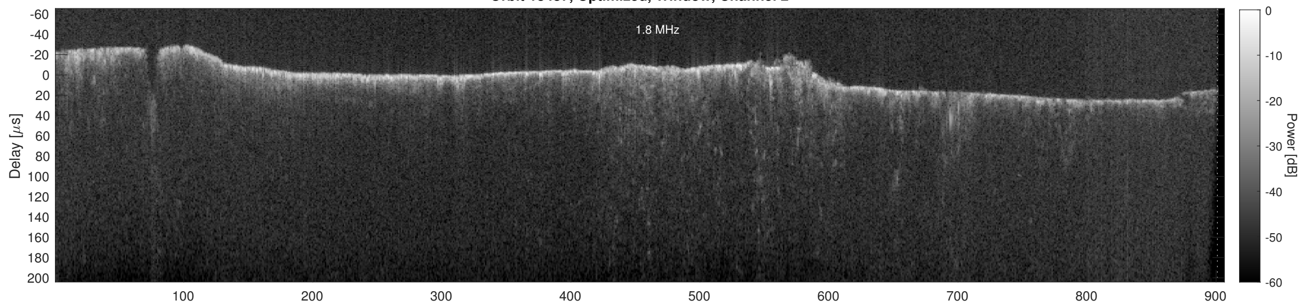
Orbit 18487, Cluttergram
