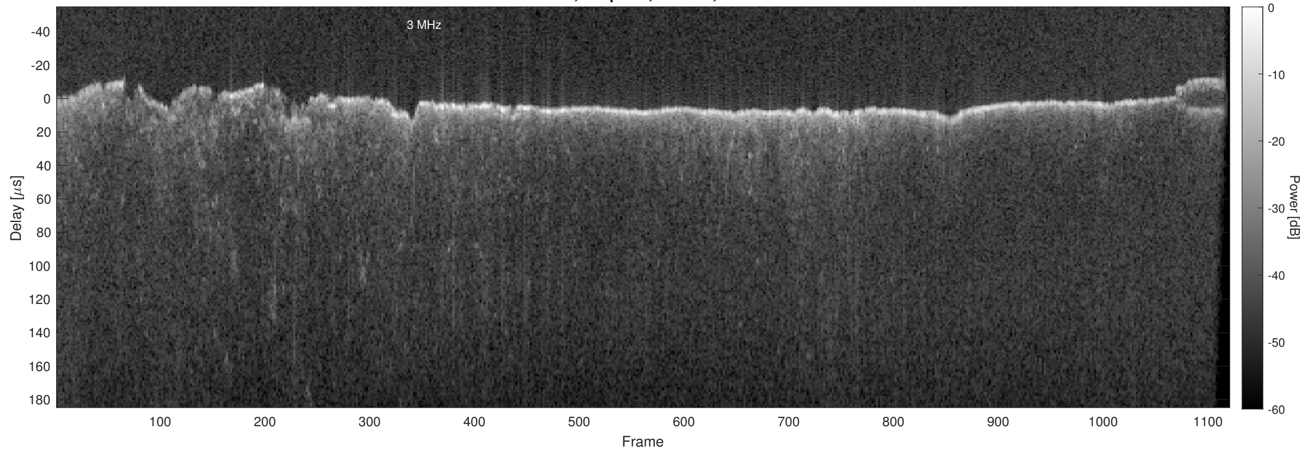
Orbit 18490, Chapman, Window, Channel 2
