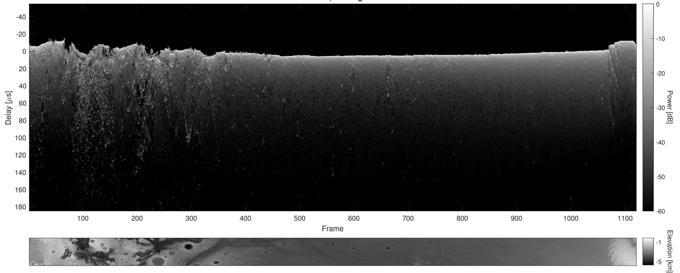
Orbit 18490, Cluttergram
