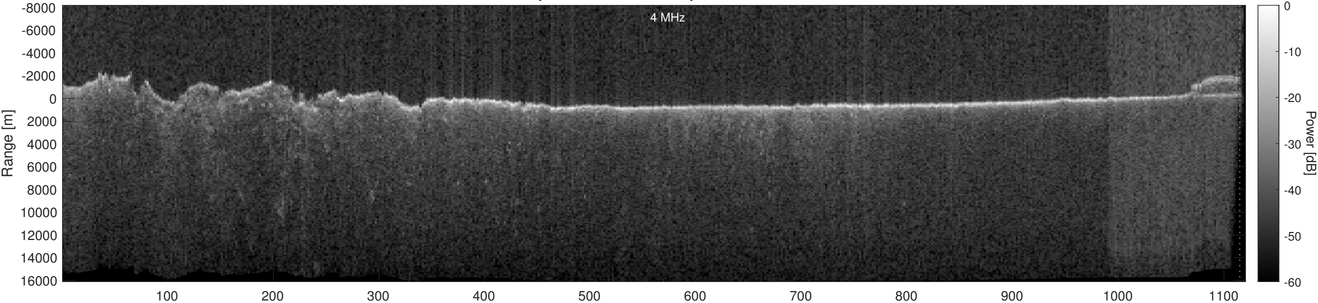
Orbit 18490, Optimized, Window, Depth-Corrected, Channel 2
