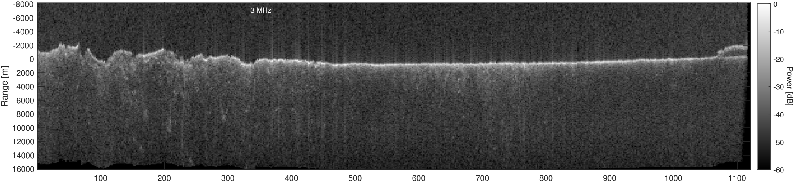
Orbit 18490, Depth-Corrected Cluttergram
