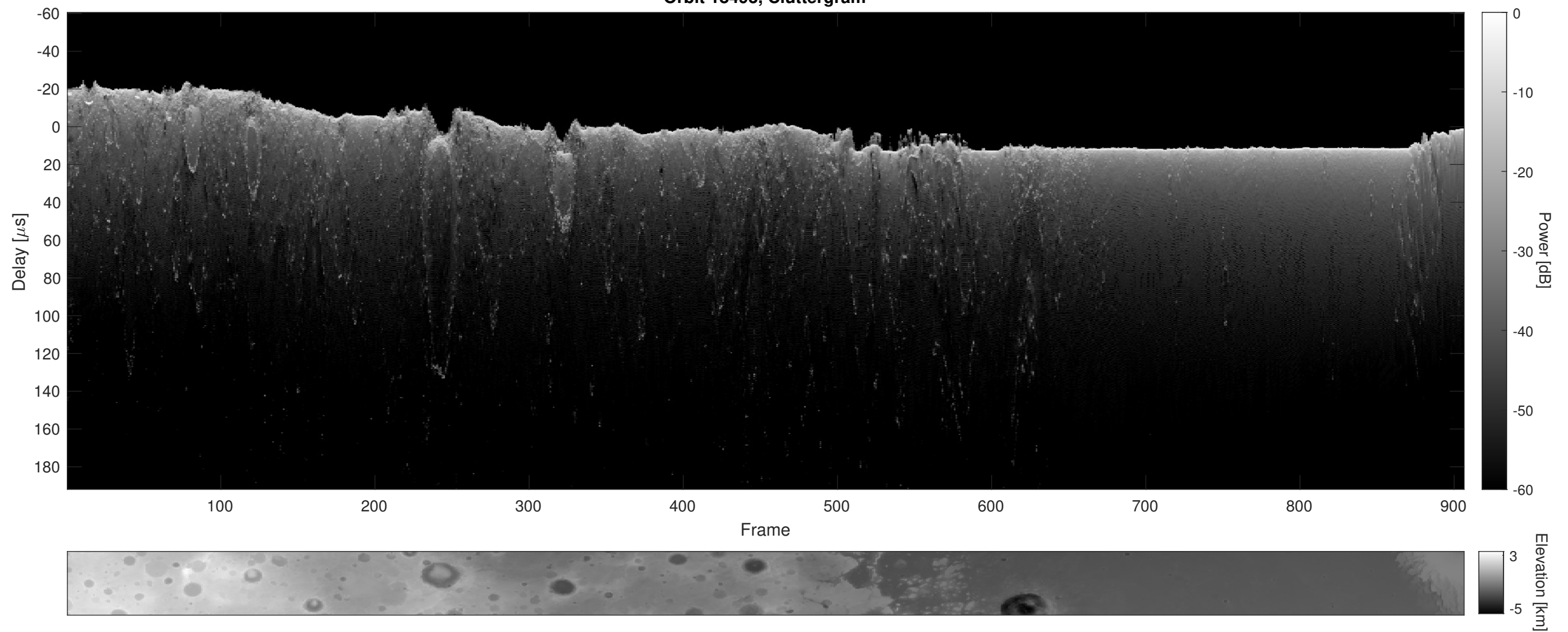
Orbit 18493, Cluttergram
