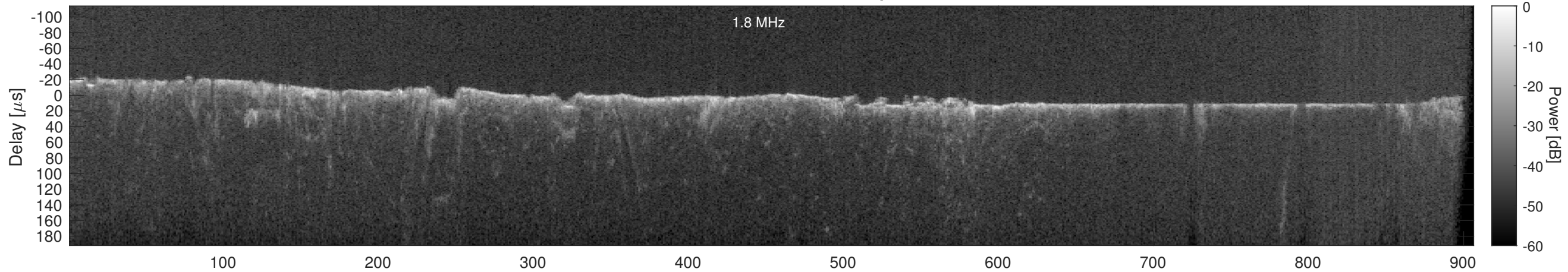
Orbit 18493, Cluttergram
