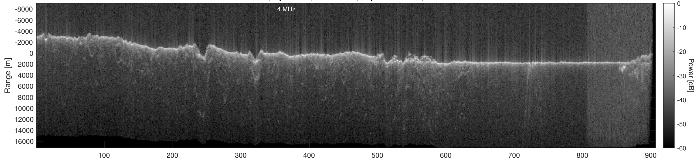
Orbit 18493, Optimized, No Window, Depth-Corrected, Channel 2
