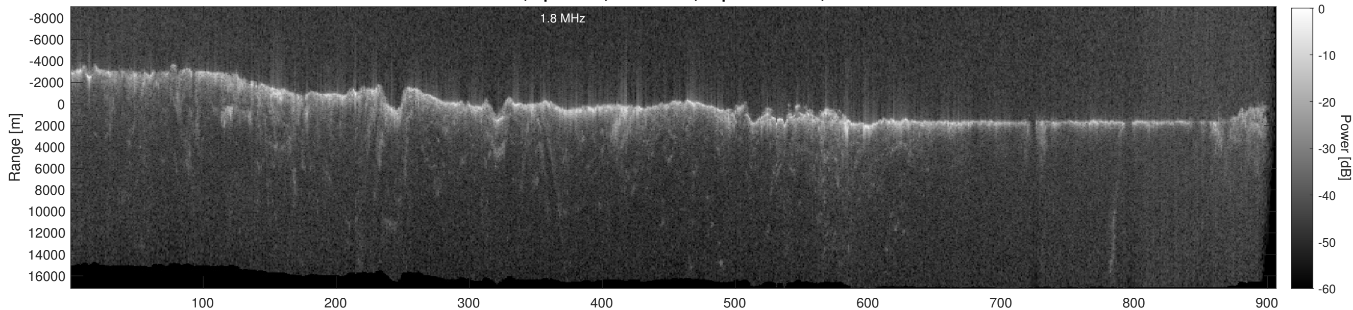
Orbit 18493, Depth-Corrected Cluttergram
