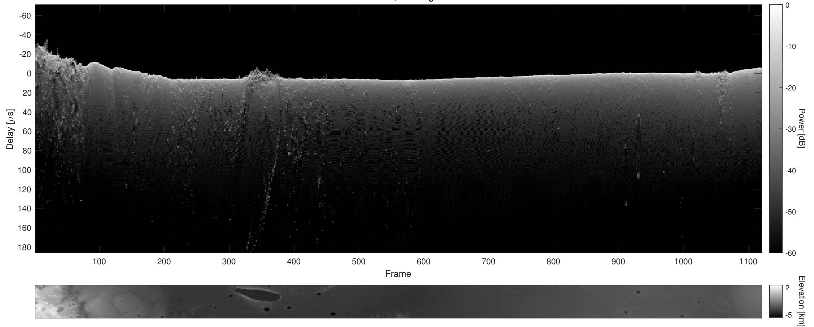
Orbit 18495, Cluttergram
