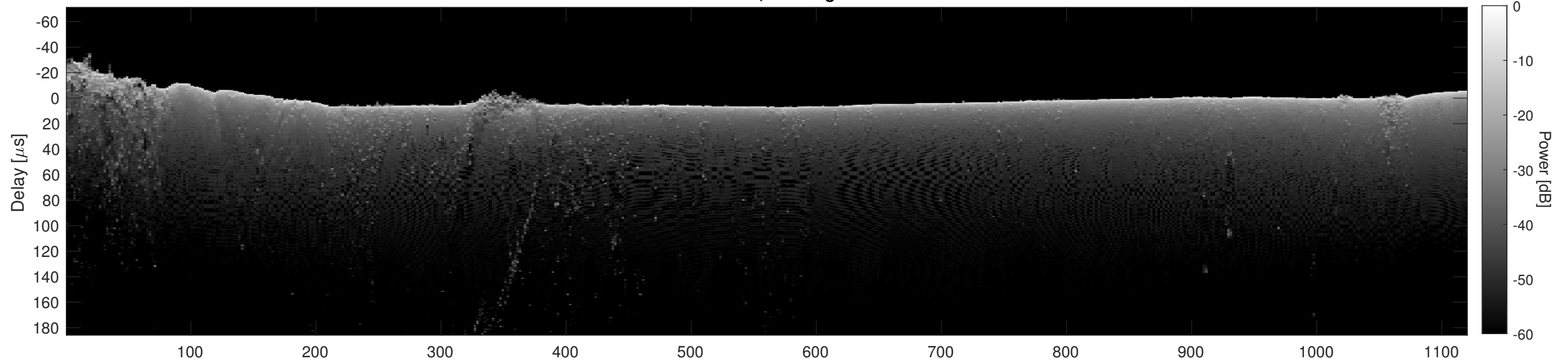
Orbit 18495, Cluttergram
