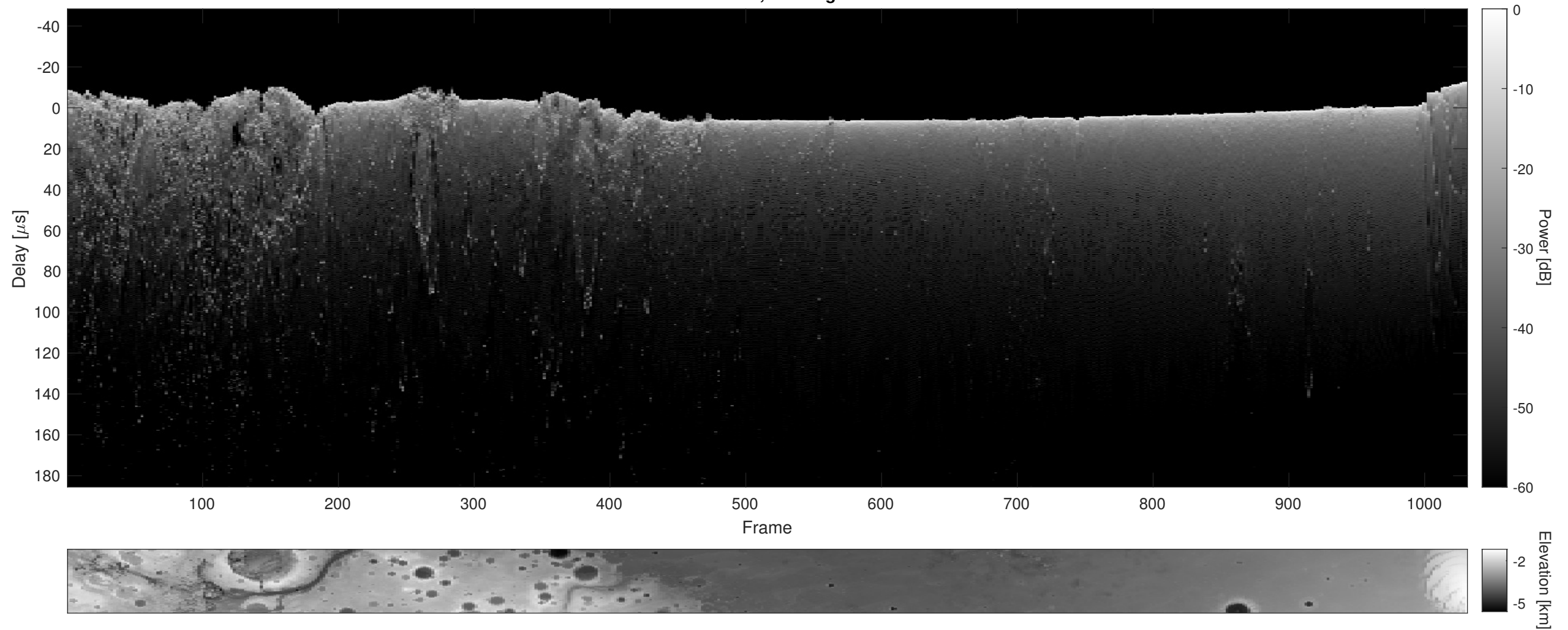
Orbit 18504, Cluttergram
