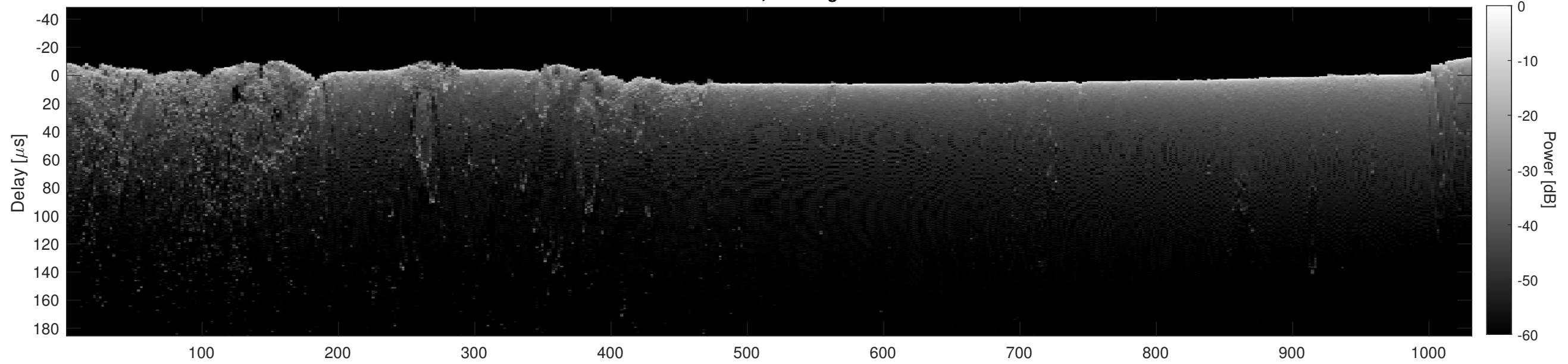
Orbit 18504, Cluttergram
