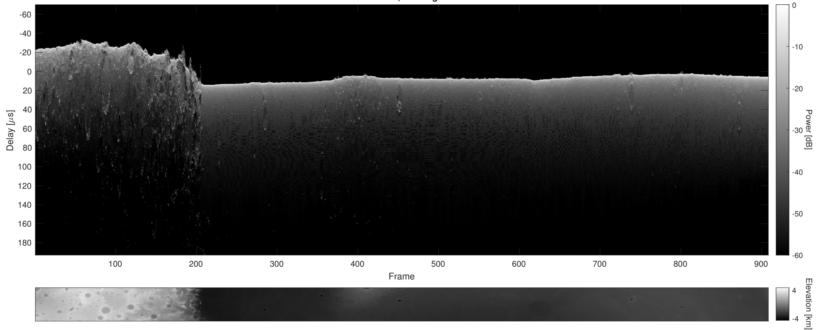
Orbit 18510, Cluttergram
