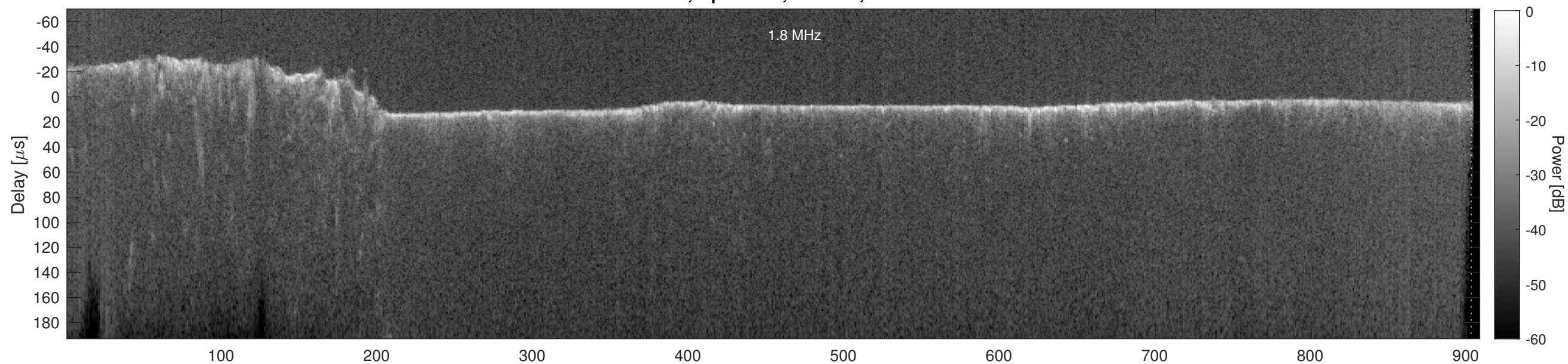
Orbit 18510, Cluttergram
