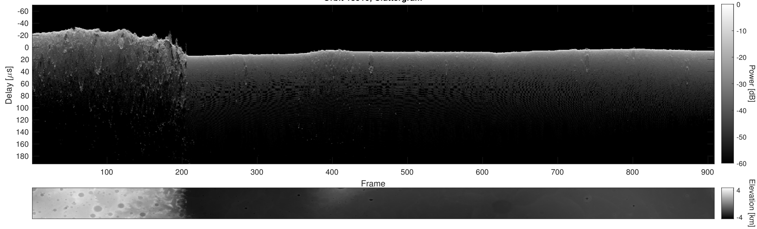
Orbit 18510, Cluttergram
