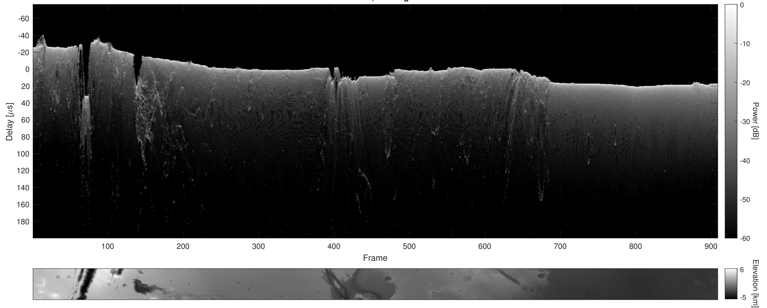
Orbit 18515, Cluttergram
