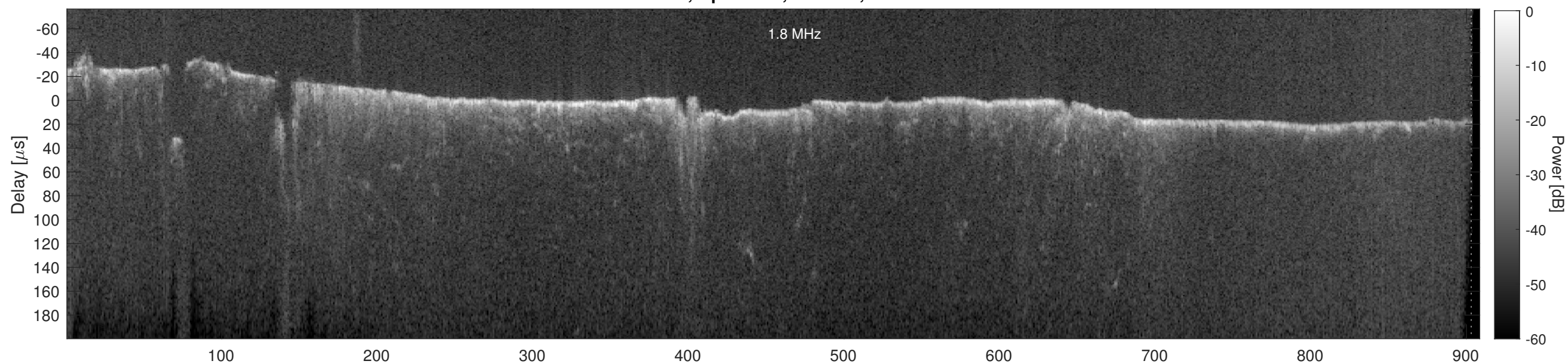
Orbit 18515, Cluttergram
