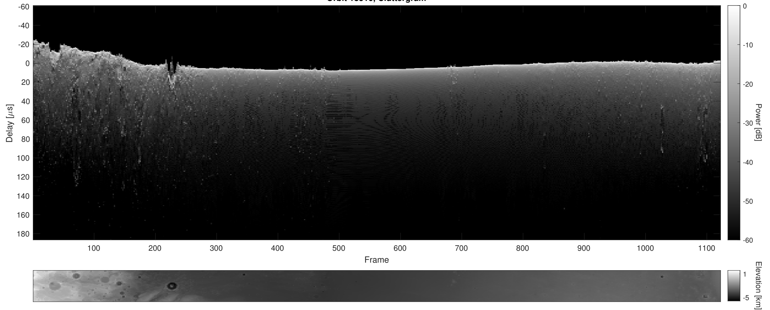
Orbit 18516, Cluttergram
